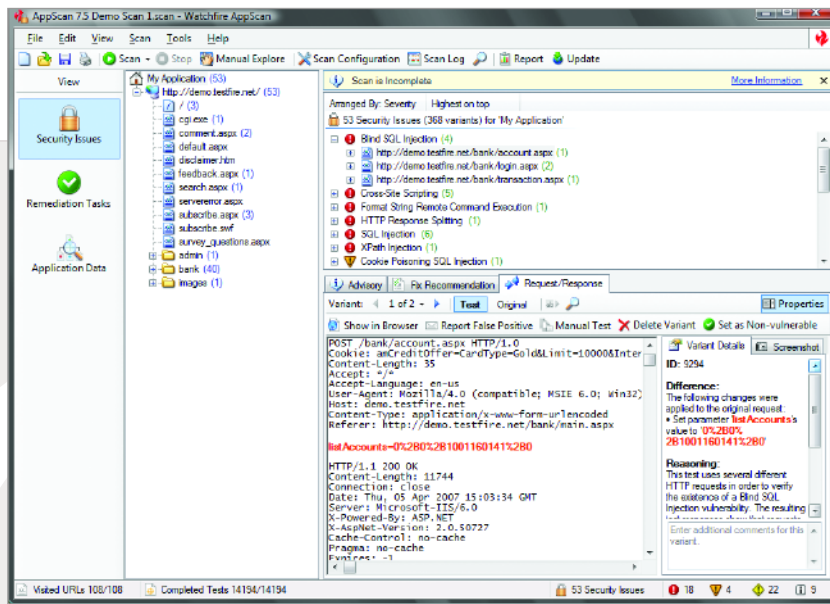
AppScan provides full details showing how vulnerabilities are exposed
